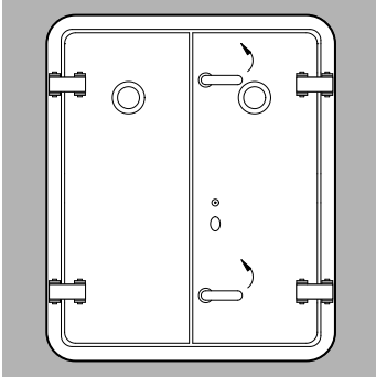
CC-3006AH - Round Light Weatherside View
