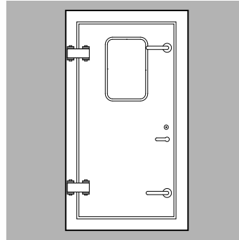
CC-3009AH - Rectangle Lite Weatherside View
